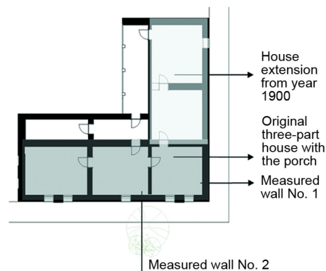
Figure 2. Ground floor plan of traditional house in Vojvodina, city of Pancevo; ground floor layout in shape of letter L; marked measured positions of the walls
