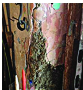
Figure 4. Rammed earth wall with a large quantity of added straw (chaff) plastered with mud mortar, house in Pancevo
