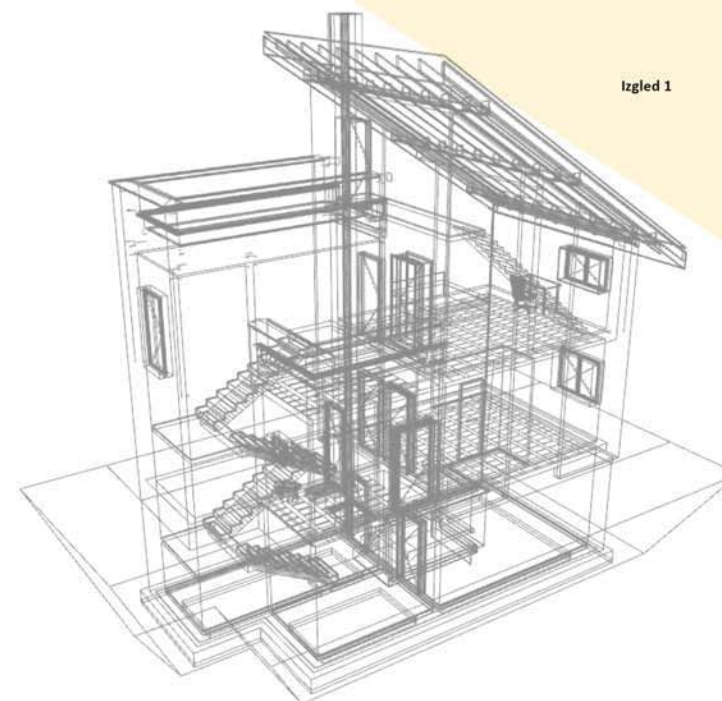
3D Model
