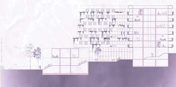
Presek 2-2 R 1:250
