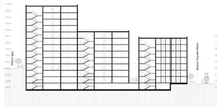
PRESEK 2-2 1:250
